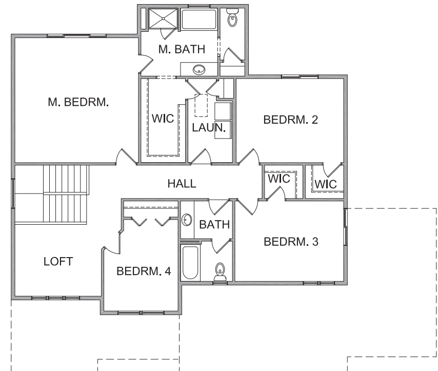
Upper Level: 1,510sf
