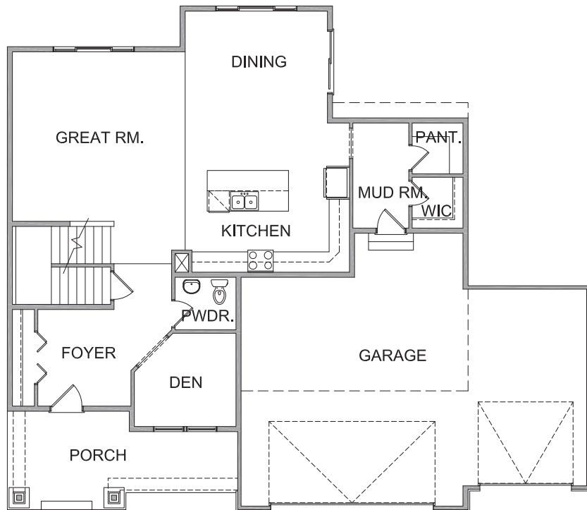
Main Level: 1,271sf
